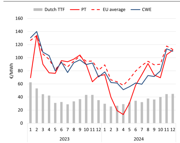
Graph A8.1: Monthly average day-ahead wholesale electricity prices and European benchmark natural gas prices (Dutch TTF)
