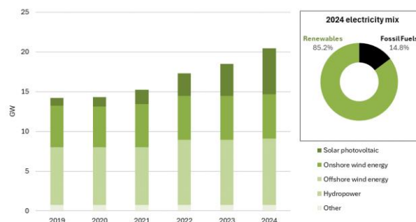
Graph A8.2: Portugal's installed renewable capacity (left) and electricity generation mix (right)
